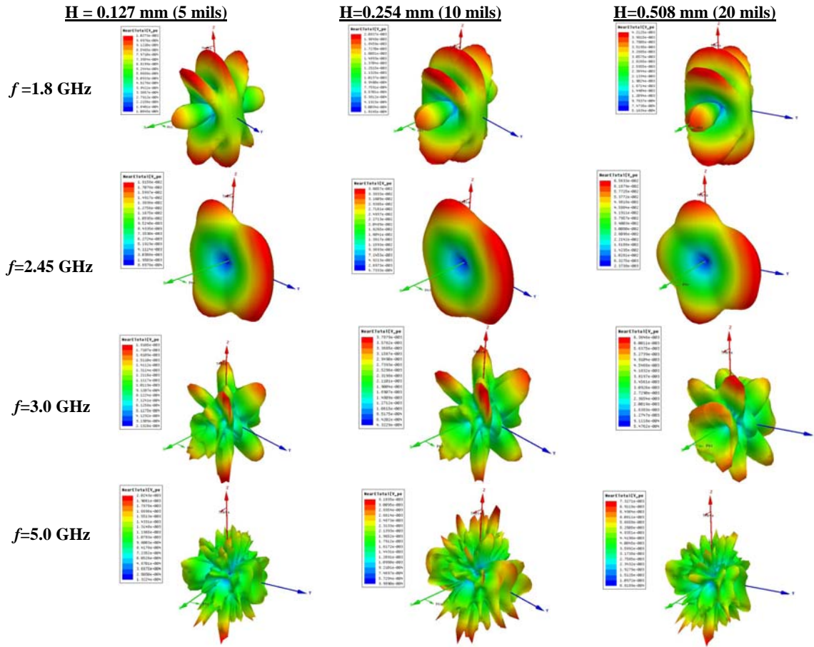
Fig. 5 Plots of the radiated field at 3-meter distance parallel to the PCB with ground stitches.
