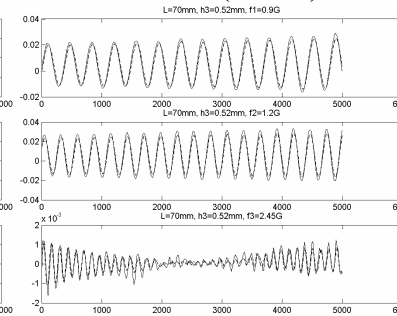
Figure 6. Poynting vector plots (for numerical data used in Tables 1, 2 and 3)
