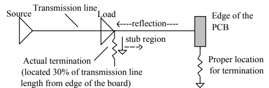
Transmission line representation of power and return planes
