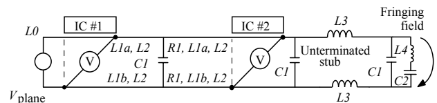
Power and ground plane mechanical equivalent representation
