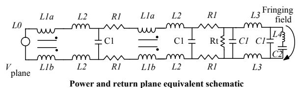
Power and return plane equivalent schematic
