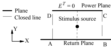
Figure 4. PCB structure for calculation Poynting vector
